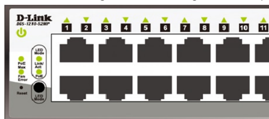
Figure 1.21 –LED Indicators on DGS-1210 series
