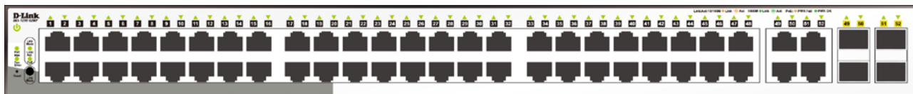
Figure 1.19 – DGS-1210-52MP Front Panel
