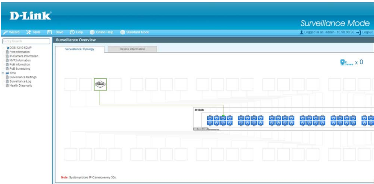
Figure 4.20 – Surveillance Mode
