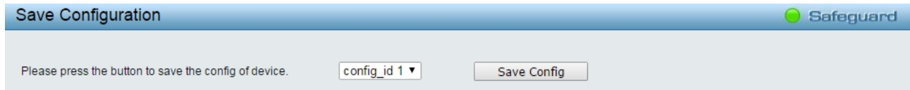
Figure 4.8 – Save Configuration
