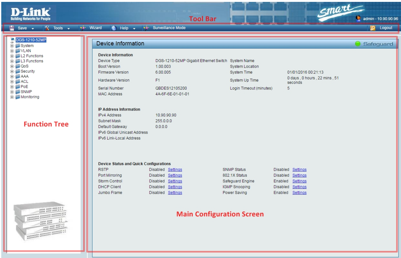
Figure 4.6 – Web-based Management
