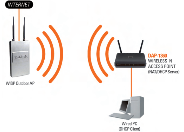
Connecting wired PCs to the Internet using the DAP-1360
