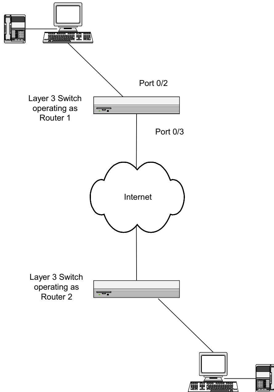
Figure 106. DiffServ VoIP Example Network Diagram
