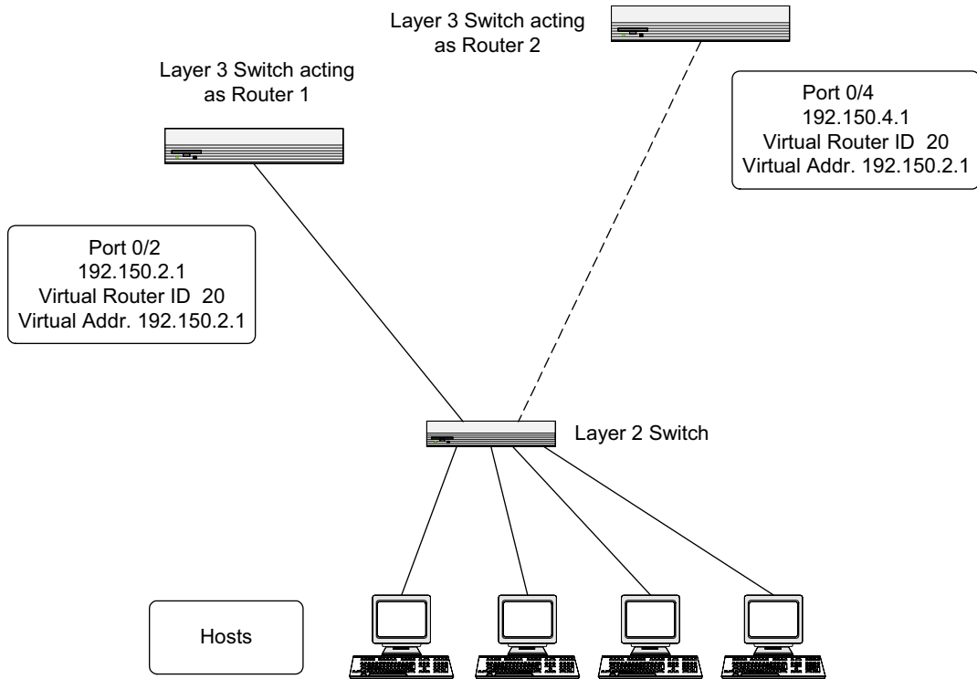
Figure 37. VRRP Example Network Configuration
