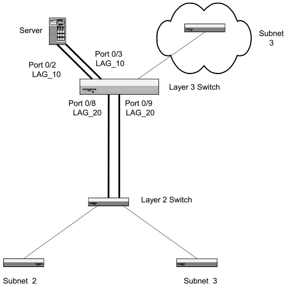
Figure 10. LAG/Port-channel Example Network Diagram
