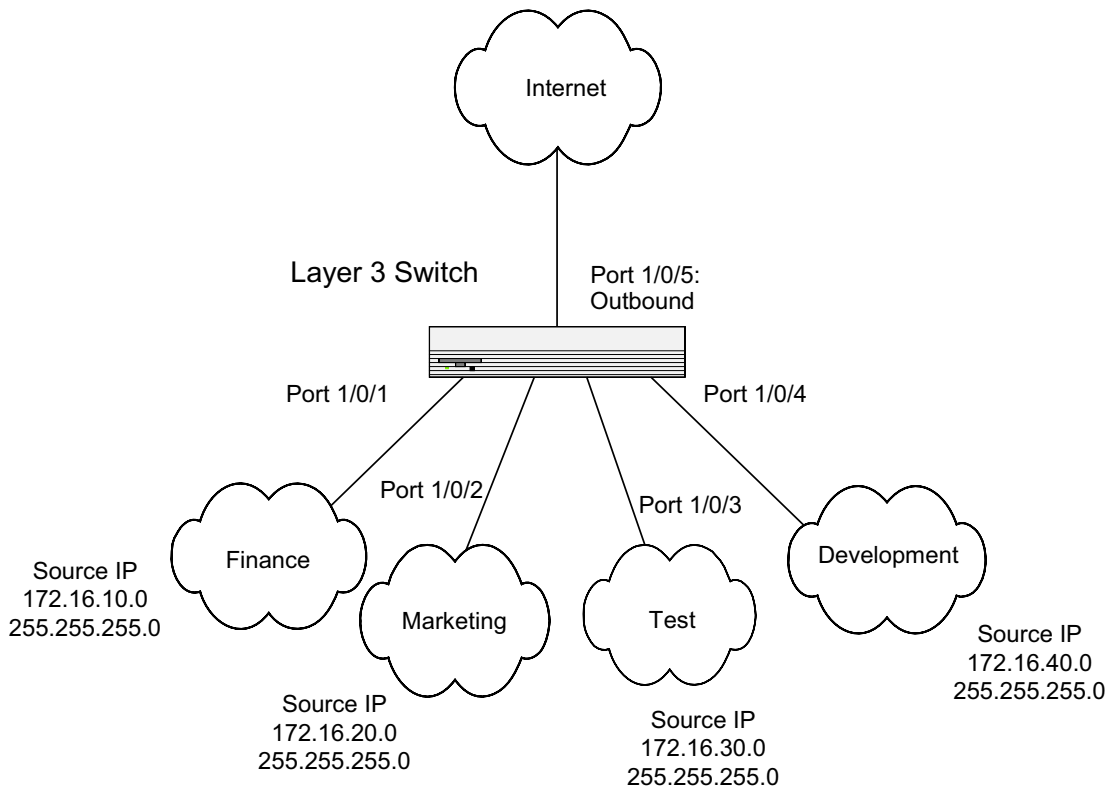
Figure 91. DiffServ Internet Access Example Network Diagram
