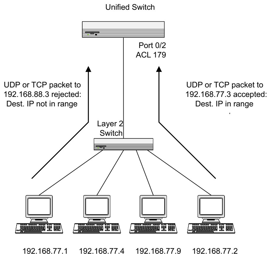
Figure 46. IP ACL Example Network Diagram
