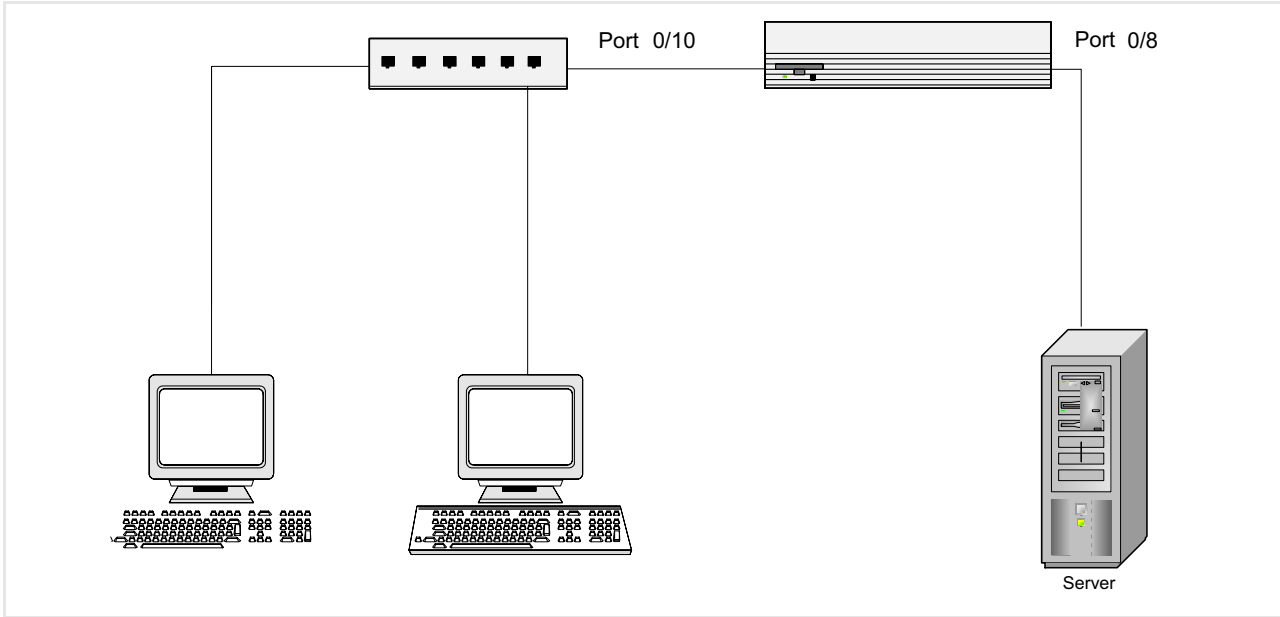
Figure 84. CoS Configuration Example System Diagram
