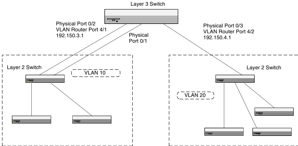
Figure 31. VLAN Routing Example Network Diagram
