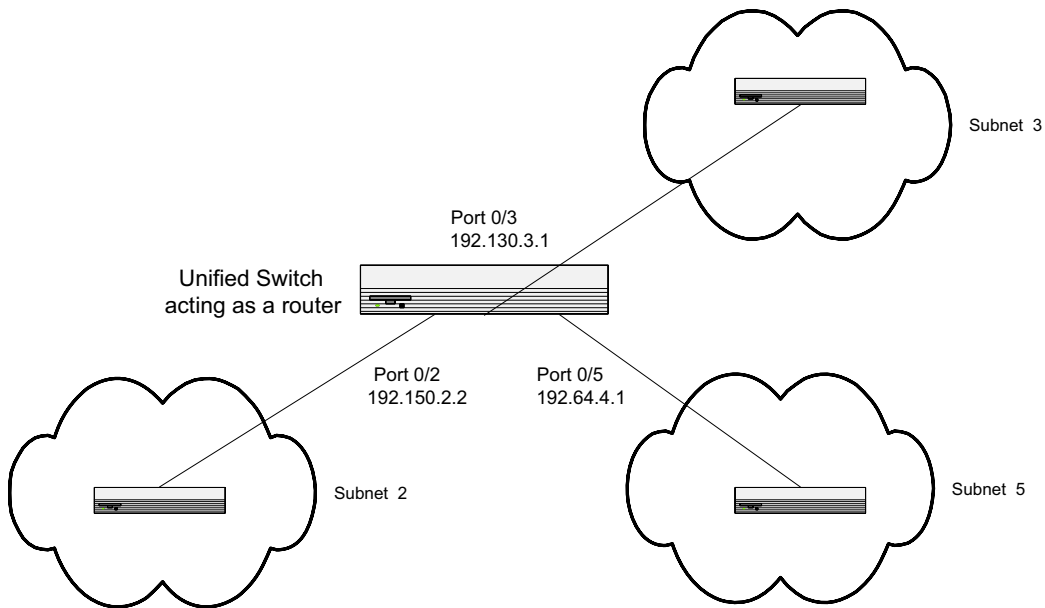
Figure 28. Port Routing Example Network Diagram
