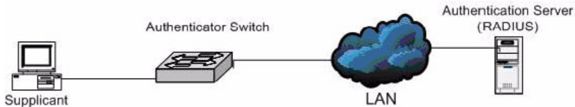
Figure 60. DWS-3000 with 802.1x Network Access Control
