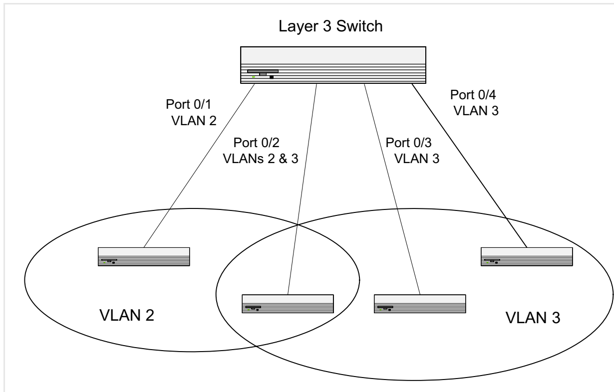
Figure 5. VLAN Example Network Diagram
